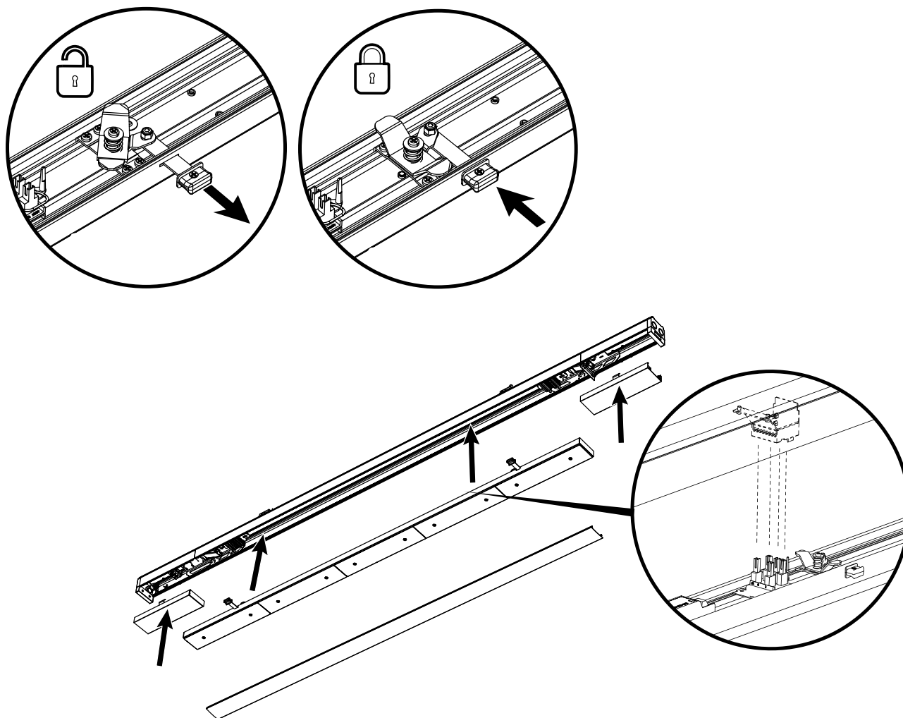
Optional blanking plate. Product code: LPMBP
